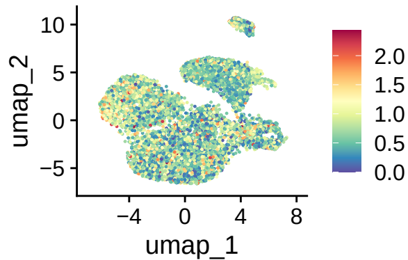
nFeature_RNA
